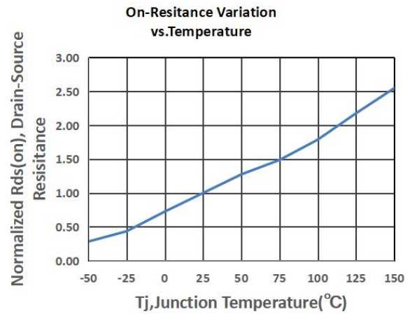
Fig2 Normalized On-Resistance Vs. Temperature
