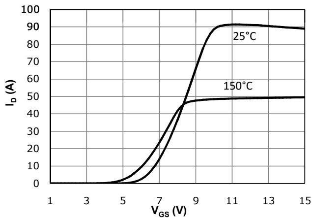
Fig 3: Transfer Characteristics
