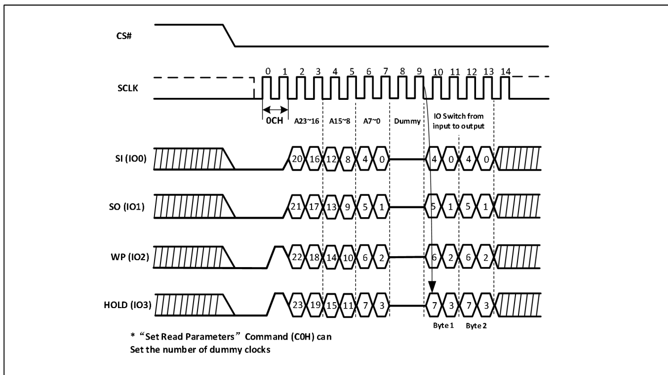
Figure 28. Burst Read with Wrap Sequence ( QPI )
