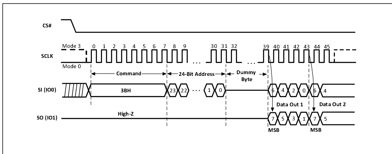
Figure-17. Dual Output Fast Read Sequence Diagram
