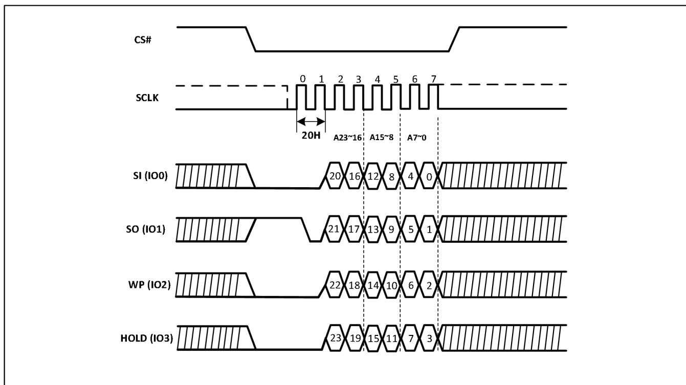
Figure-33. Sector Erase Sequence Diagram (QPI)
